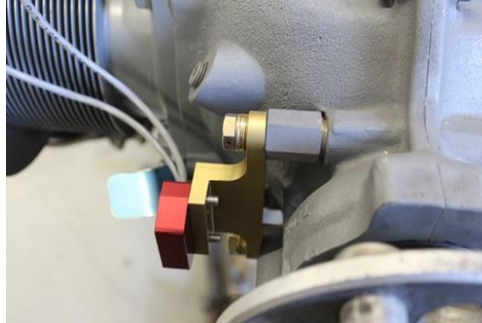
Standoff detail
